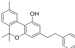
C-0117 Bibenzyl cannabinol, 6,6,9-Trimethyl-3-phenethyl-6H-benzo[c]chromen-1-ol C 24 H 24 O 2 ; F.W: 344.45
