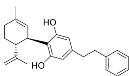
C-0107 R,R-Bibenzyl cannabidiol, 2-((1R,6R)-3-Methyl-6-(prop-1-en-2-yl)cyclo-hex-2-enyl)-5-phenethylbenzene-1,3-diol C 24 H 28 O 2 ; F.W: 348.48; [120467-09-6]
