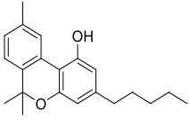
C-0053 Cannabinol, 6,6,9-trimethyl-3-pentyl-6H- benzo[c]chromen-1-ol C 21 H 26 O 2 ; F.W: 310.43
