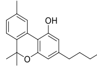
C-0056 Cannabinol-C4, 3-butyl-6,6,9-trimethyl-6H- benzo[c]chromen-1-ol C 20 H 24 O 2 ; F.W: 296.40
